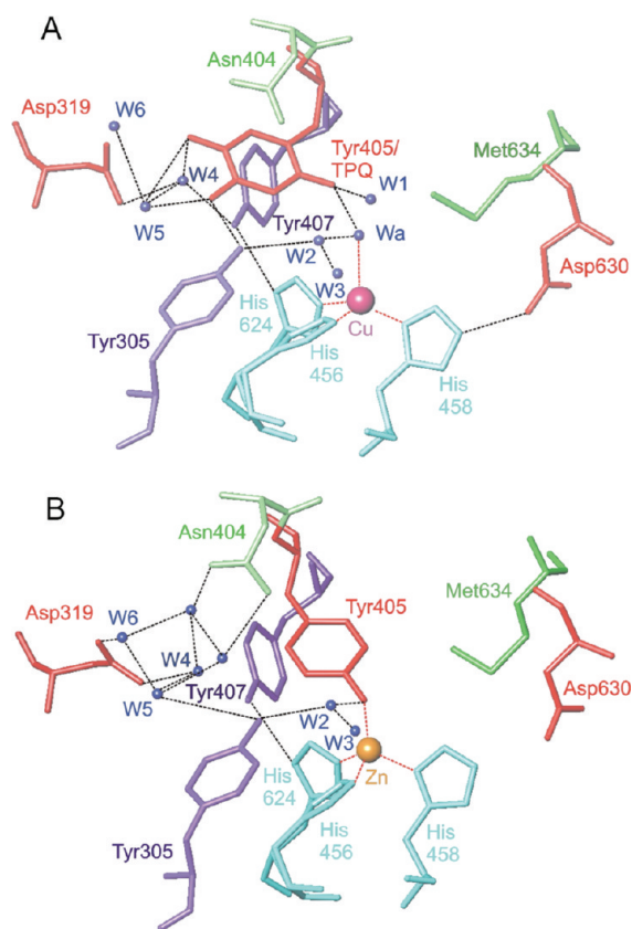
FIGURE 1: (A) Mature HPAO active site with TPQ in the reactive conformation (6). Acidic side chains are in red, basic are in cyan, aromatic are in purple, neutral hydrophilic are in lime, the TPQ is in red, and the Cu(II) ion is in crimson. A network of six active site water molecules (W1–W6) and one axial copper-coordinating water (Wa) that forms hydrogen bonds to TPQ and side chain atoms (6) are shown in blue. A seventh water, We, is also coordinated to the Cu(II) ion but is not shown. Hydrogen and metal coordination bonds are shown as black and red dashed lines, respectively. (B) Precursor HPAO active site (26), Zn(II) (gold), and unmodified Tyr405 (red). The color schemes for atoms and coordination or hydrogen bonds are as in (A) (these figures are reprinted with permission from ref 8).
