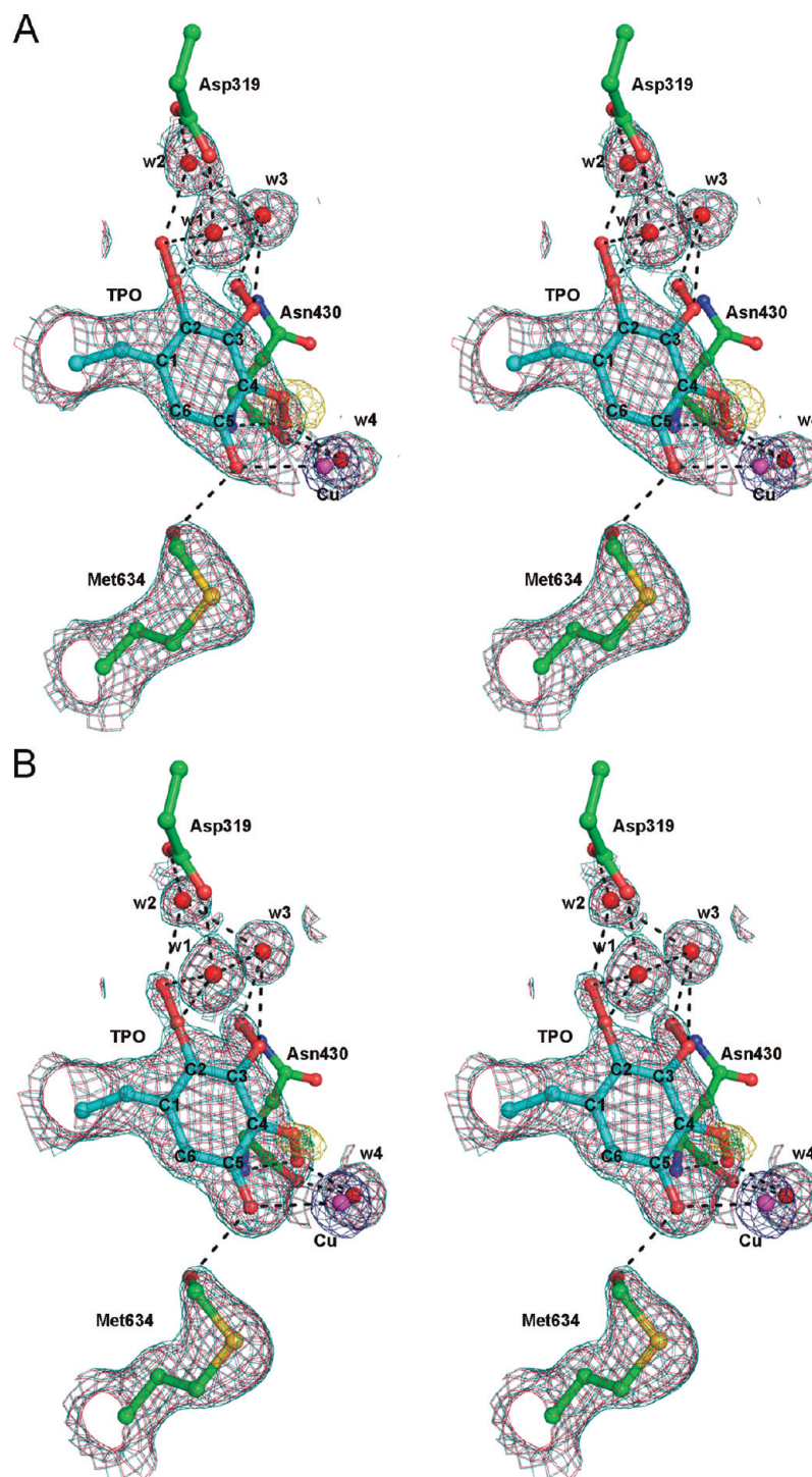
FIGURE 4: Final electron density maps of the Y305F mutants of HPAO computed using coefficients (2F_o - F_c) and (F_o - F_c) where F_c was calculated from the models refined with TPO and the modified Met634 present. The (2F_o - F_c) maps are contoured at the 0.8 (cyan), 1.0 (crimson), and 8.0 (dark blue) \sigma levels, and the (F_o - F_c) maps are contoured at the -3.0\sigma level (gold); no contours above the +3.0\sigma level are present. Contours are drawn for the TPO and modified Met634 side chains, as well as for waters, w1–w4. The side chains of Asp319 and Asn430 are also shown without contours (for clarity). Hydrogen and coordination bonds are indicated by black dashed lines. The atom coloring and numbering scheme is the same as in Figure 3 with the additional numbering of four water molecules, w1–w4. These four waters correspond closely to the active site waters found in the native and Y305A structures, namely, waters w4, w7, w5, and w3, respectively. The residues, waters, and cofactor oxygen atoms are labeled. (A) The E. coli -expressed structure is shown. (B) The yeast-expressed structure is shown.
