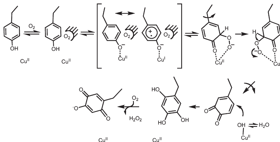
Scheme 1: Proposed Mechanism for the Biogenesis of TPQ
