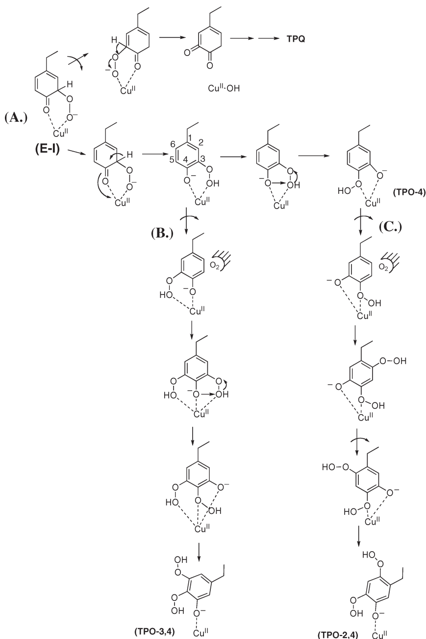
Scheme 2: (A) Mechanism for Branching of a Biogenesis Intermediate to TPQ and TPO, (B) Model To Explain Partial Occupancy of a Derivative at C-3 via Formation of TPO-3,4, and (C) Model To Explain Partial Occupancy of a Derivative at C-2 via Formation of TPO-2,4
