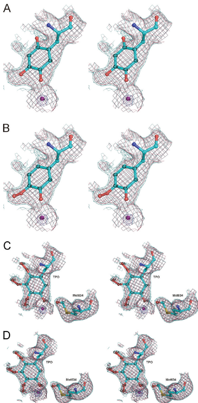
FIGURE 3: Simulated annealing omit maps of the Y305F mutants of HPAO computed using coefficients ( F_o - F_c ) where F_c were calculated from models in which the side chain of residue 405 was absent; in panels A–C F_o were the structure factors observed from crystals of the E. coli -expressed mutant and in panel D from the yeast-expressed mutant. The maps are contoured at \sigma levels of 2.5 (cyan), 3.0 (crimson), and 10.0 (purple). Atoms are colored blue for nitrogen, red for oxygen, and magenta for copper; for the residue 405 cofactor, the carbon atoms are in cyan. (A) Stereoview of a model of TPO is shown superimposed on the omit map. (B) Stereoview of an initial model of TPO is superimposed on the map. (C, D) Stereoviews of the final model of TPO superimposed on the E. coli - and yeast-expressed simulated annealing omit maps, respectively, of the Y305F mutants. In addition, the modified methionine at position 634 (also omitted during the omit map calculation) is shown superimposed on its density.
