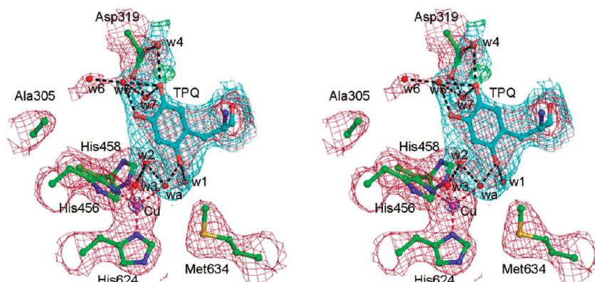
FIGURE 2: A stereoview of the Y305A mutant of HPAO. The (2F_o - F_c) electron density map (red contours at the 1\sigma level, dark blue at the 8\sigma level) and the (F_o - F_c) electron density (green contours at the +3\sigma level) are shown (no contours are present at the -3\sigma level). Also shown is the 6-fold averaged simulated annealing (F_o - F_c) omit map (cyan contours at the +3\sigma level). Carbon atoms are in green except for TPQ where carbon atoms are in cyan; nitrogen atoms are in blue, oxygen in red, sulfur in yellow, and copper in magenta. Hydrogen bonds are shown as dashed black lines and coordination bonds as dashed crimson lines. All of the active site water molecules present in the wild-type structure are shown (wa, w1–w6, shown in Figure 1A, plus an additional water, w7). Water we, present in the wild-type structure, is not visible in the Y305A mutant.
